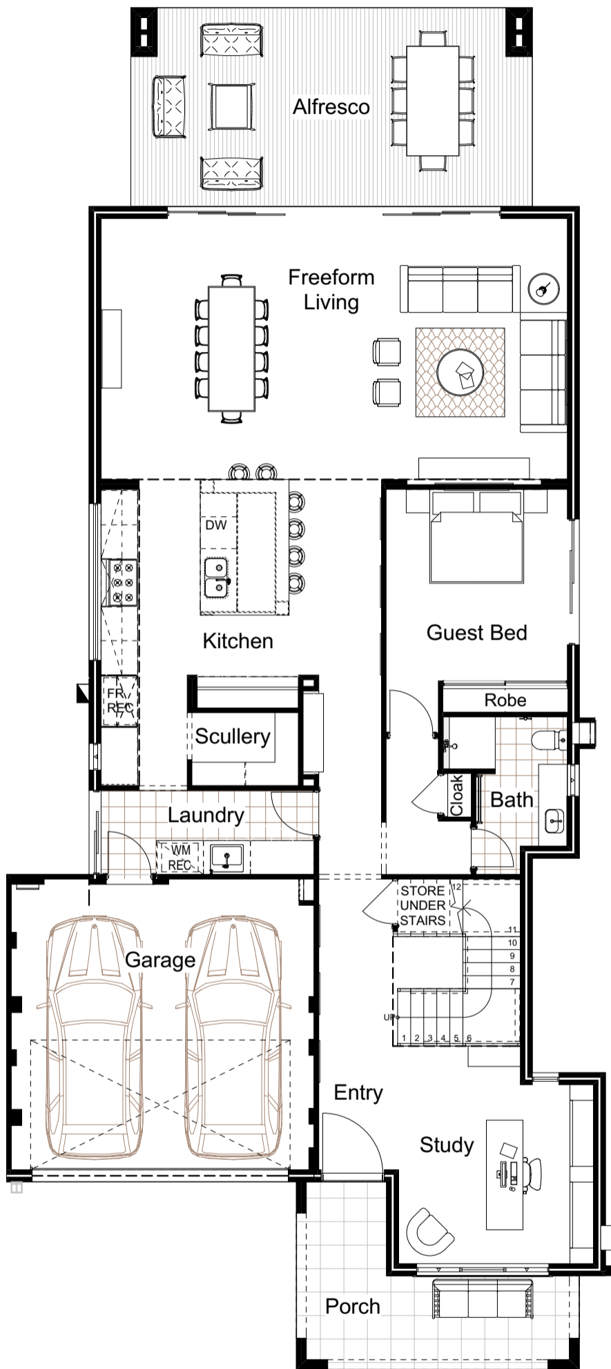
GROUND FLOOR PLAN TOTAL AREA: 418m 2
