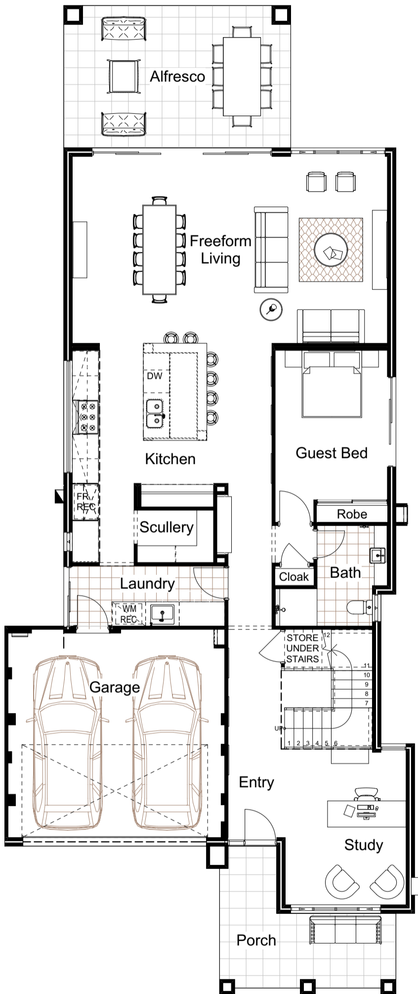
GROUND FLOOR PLAN TOTAL AREA: 347m 2
