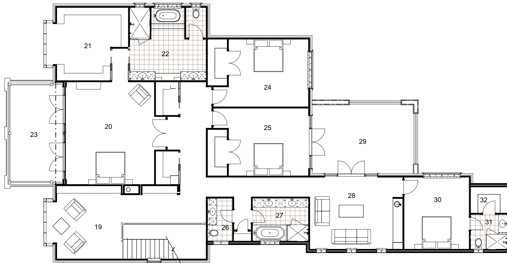
UPPER FLOOR PLAN
