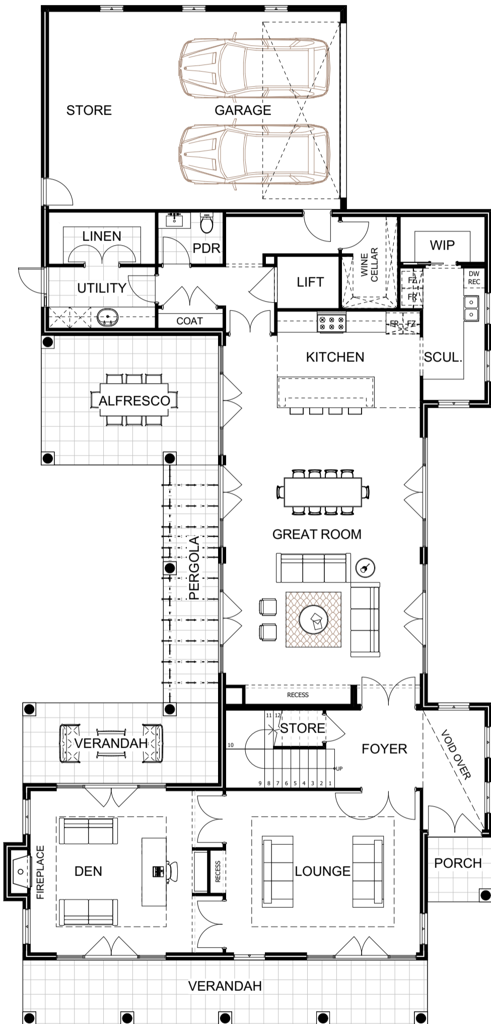
GROUND FLOOR PLAN TOTAL AREA: 595m 2
