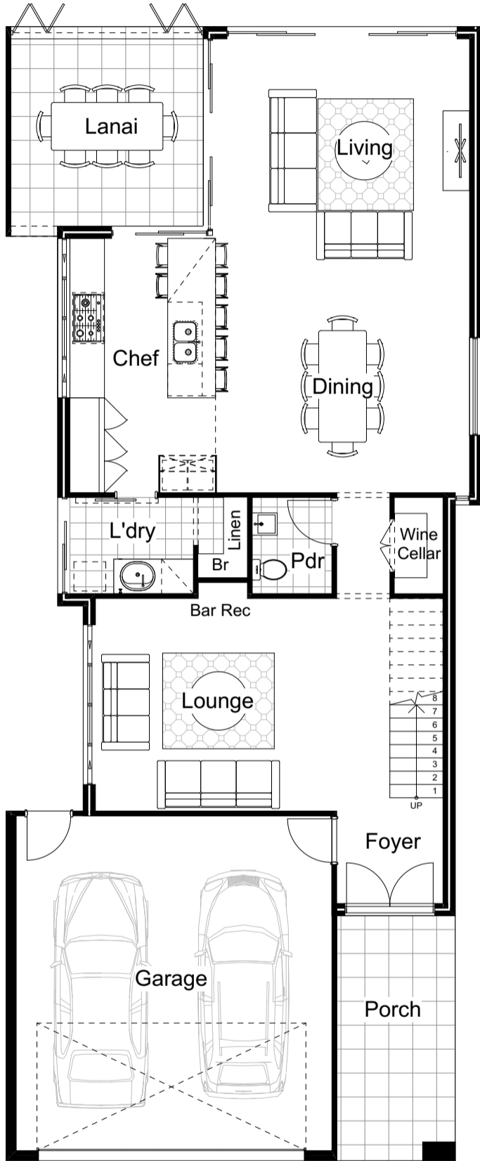
GROUND FLOOR PLAN TOTAL AREA: 290m 2
