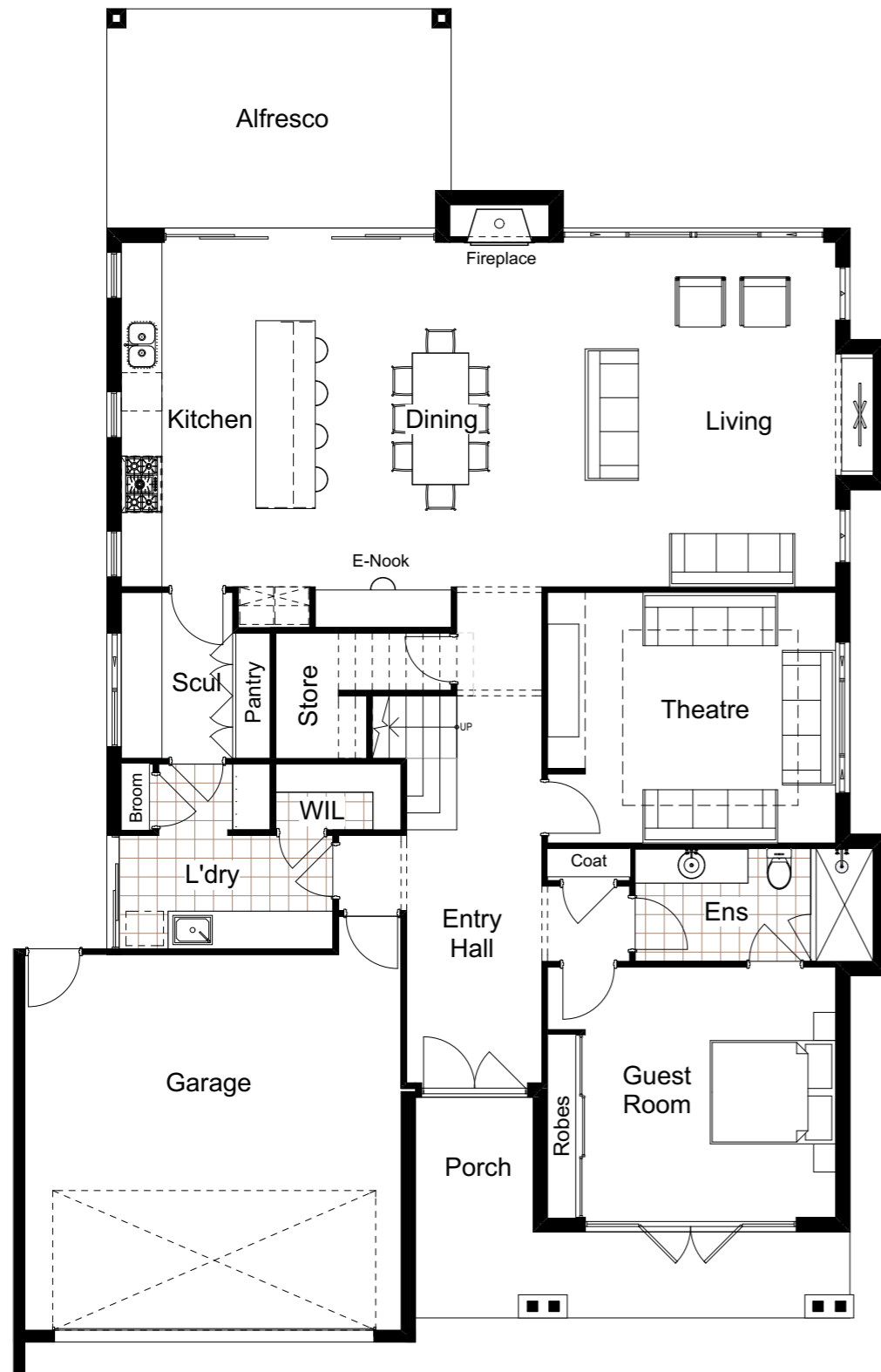
GROUND FLOOR PLAN TOTAL AREA 363m 2
