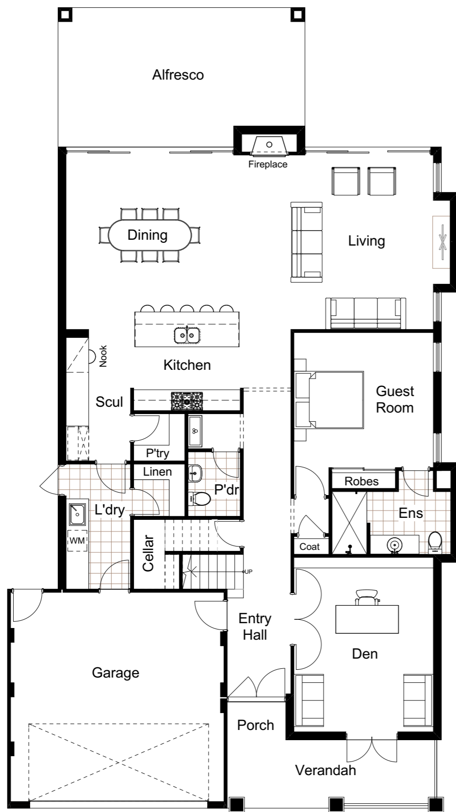
GROUND FLOOR PLAN TOTAL AREA 378m 2
