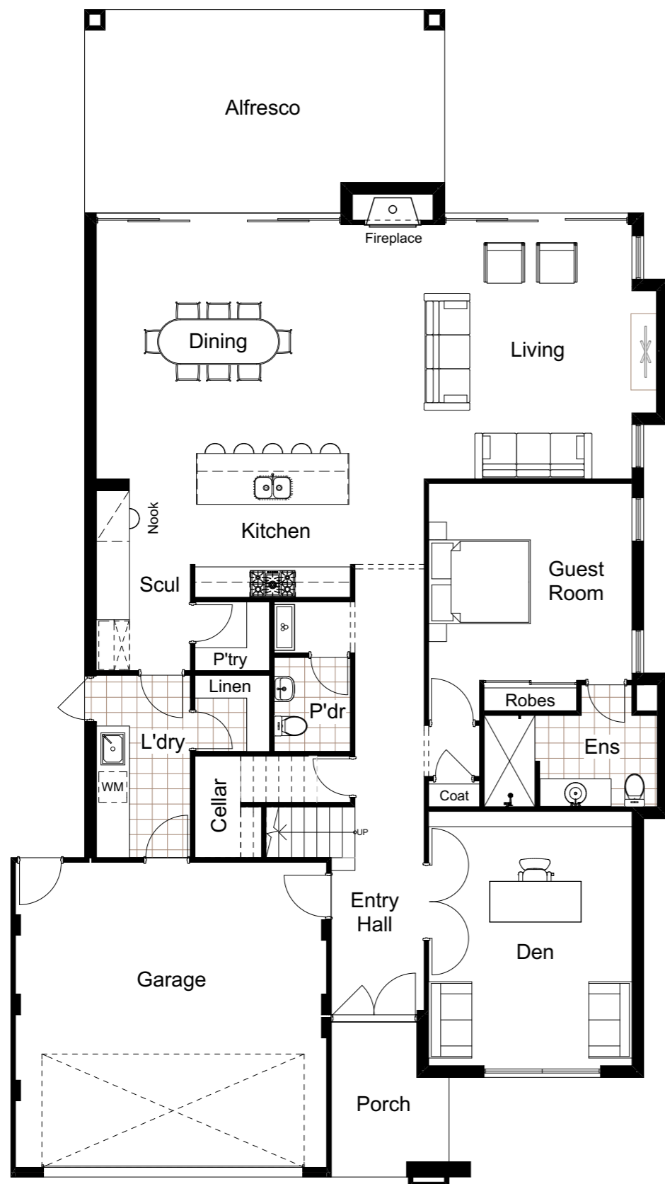
GROUND FLOOR PLAN TOTAL AREA 363m 2
