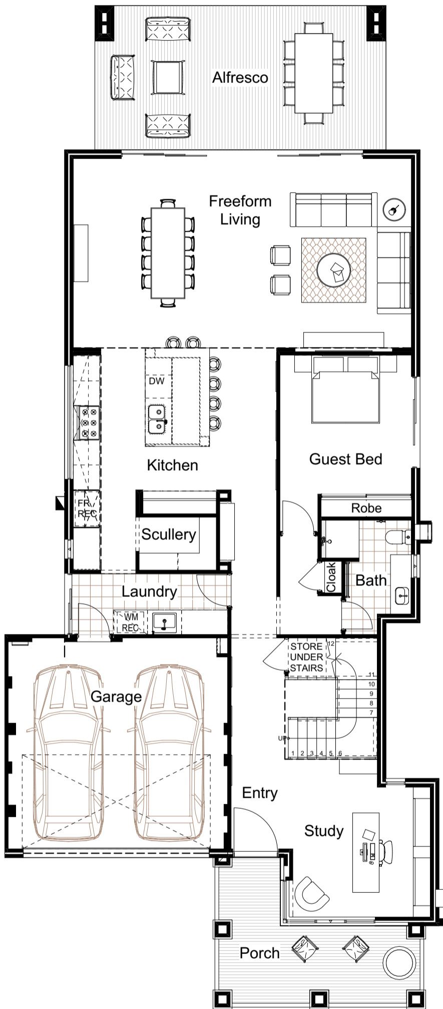
GROUND FLOOR PLAN TOTAL AREA: 422m 2
