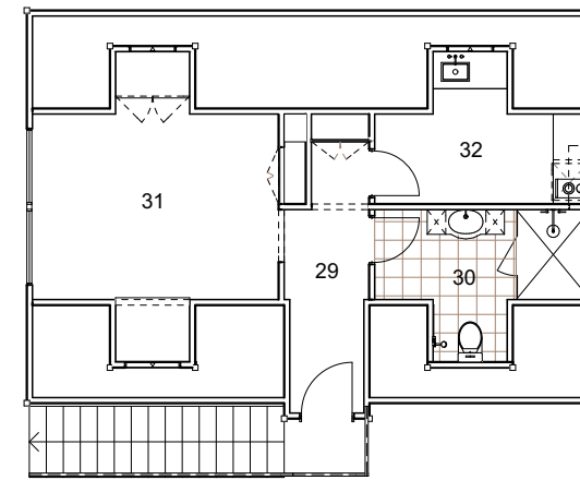
STUDIO FLOOR PLAN
